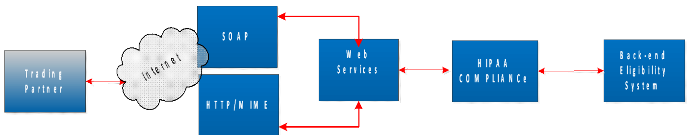
Figure 2: Transaction Process
